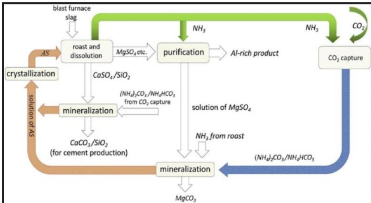
Figure 3: Carbonation of minerals with blast furnace slag
