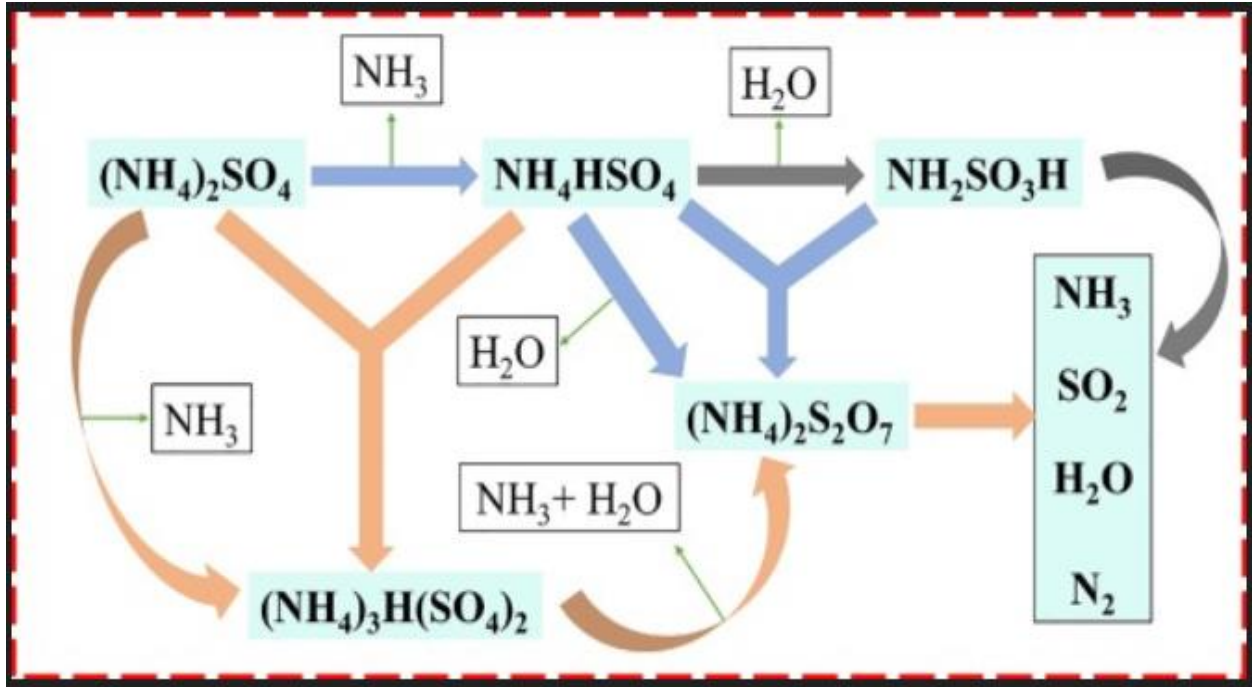
Figure 2: Process of thermal decomposition (Ammonium sulphate)
